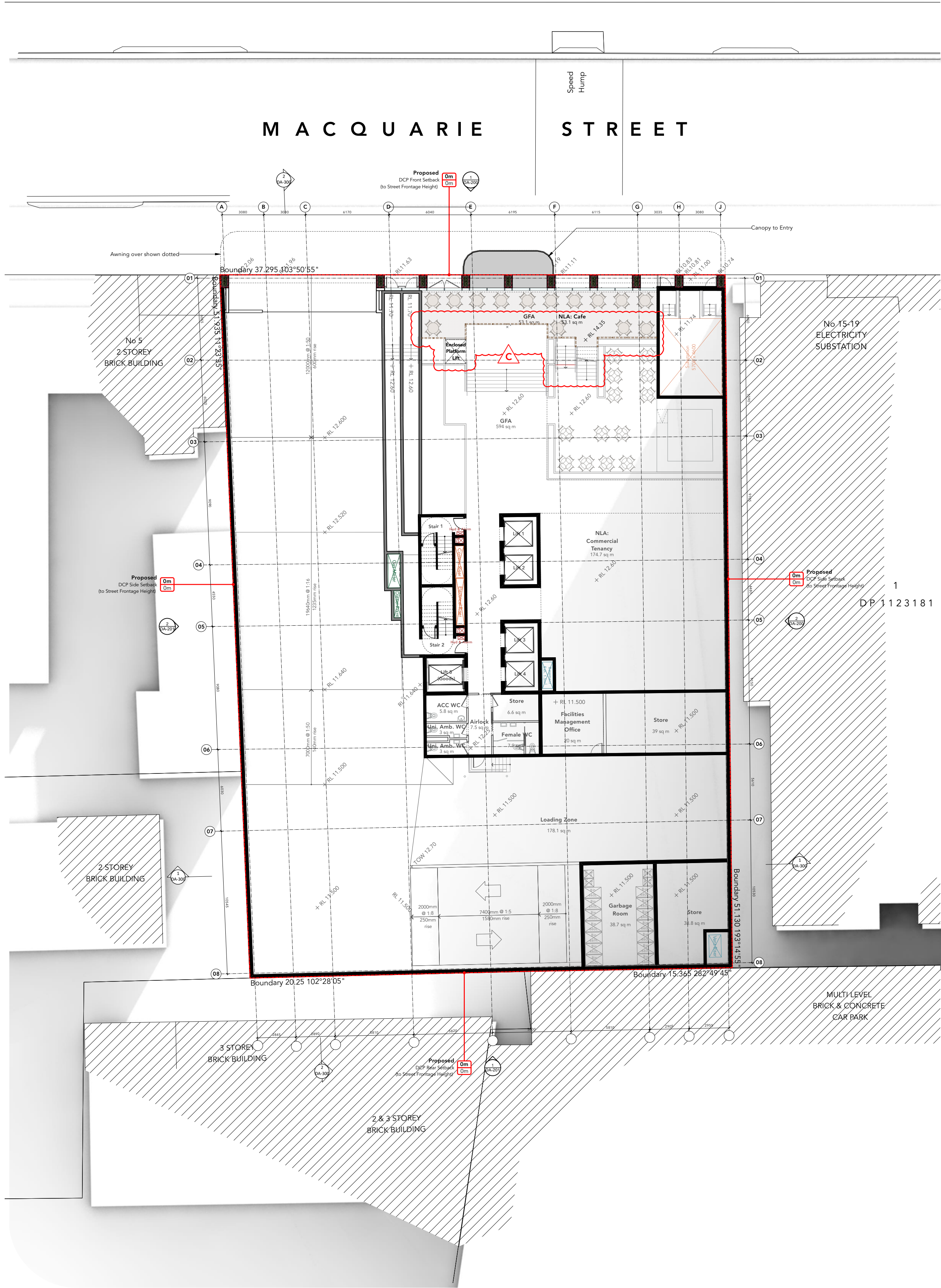
1 Plan-Ground-Level 1 Scale: 1:200
