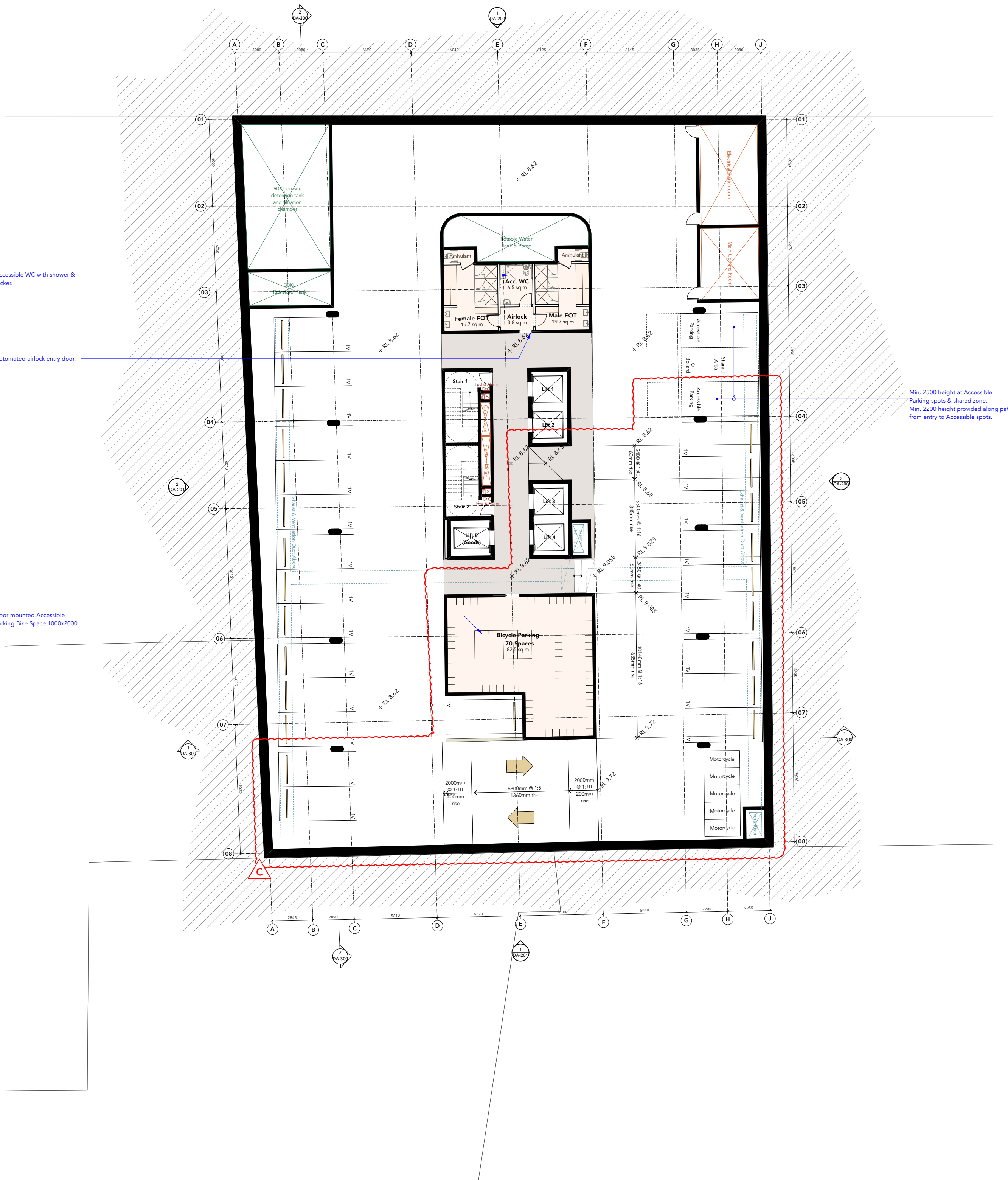
2 Plan-Basement-Level -1 Scale: 1:200
