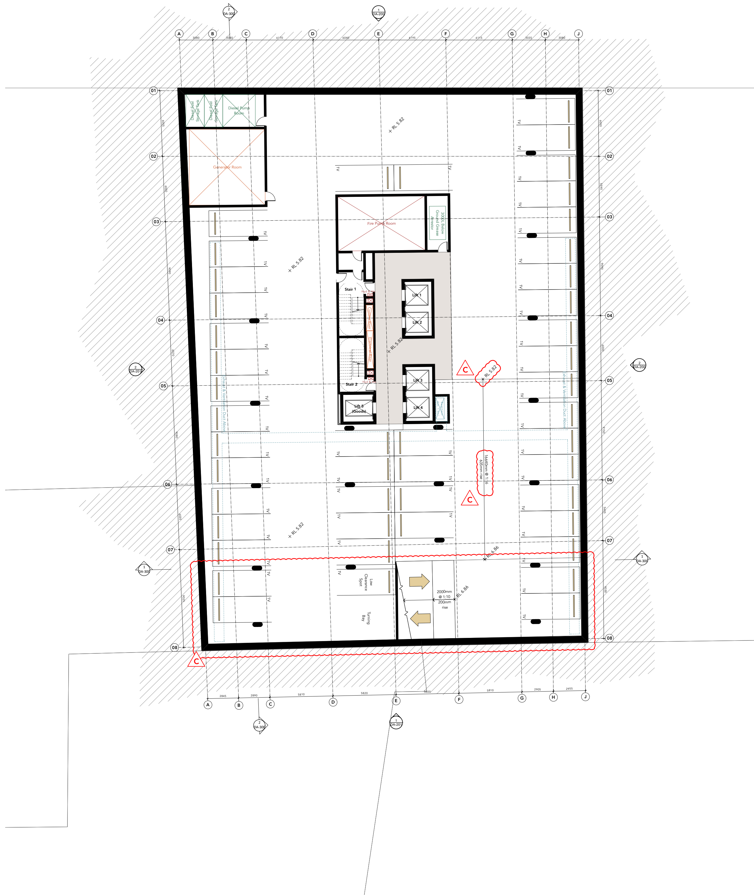
1 Plan-Basement-Level -2 Scale: 1:200
