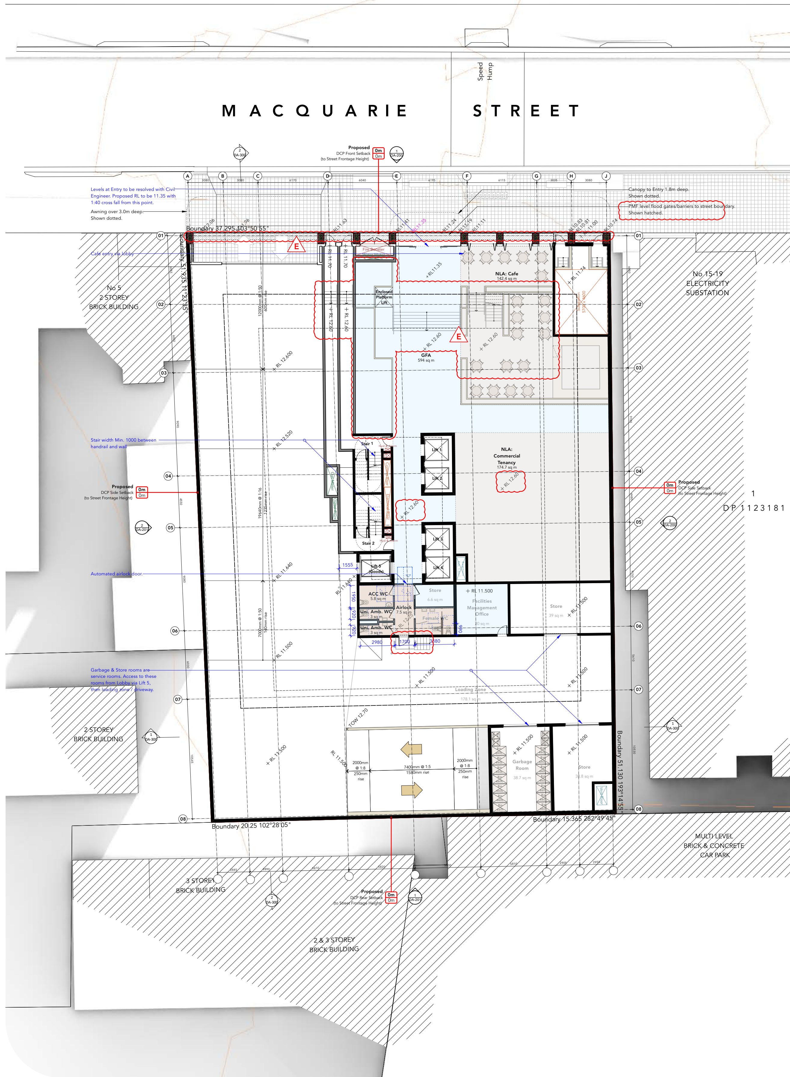
1 Plan-Ground-Level 0 Scale: 1:200
