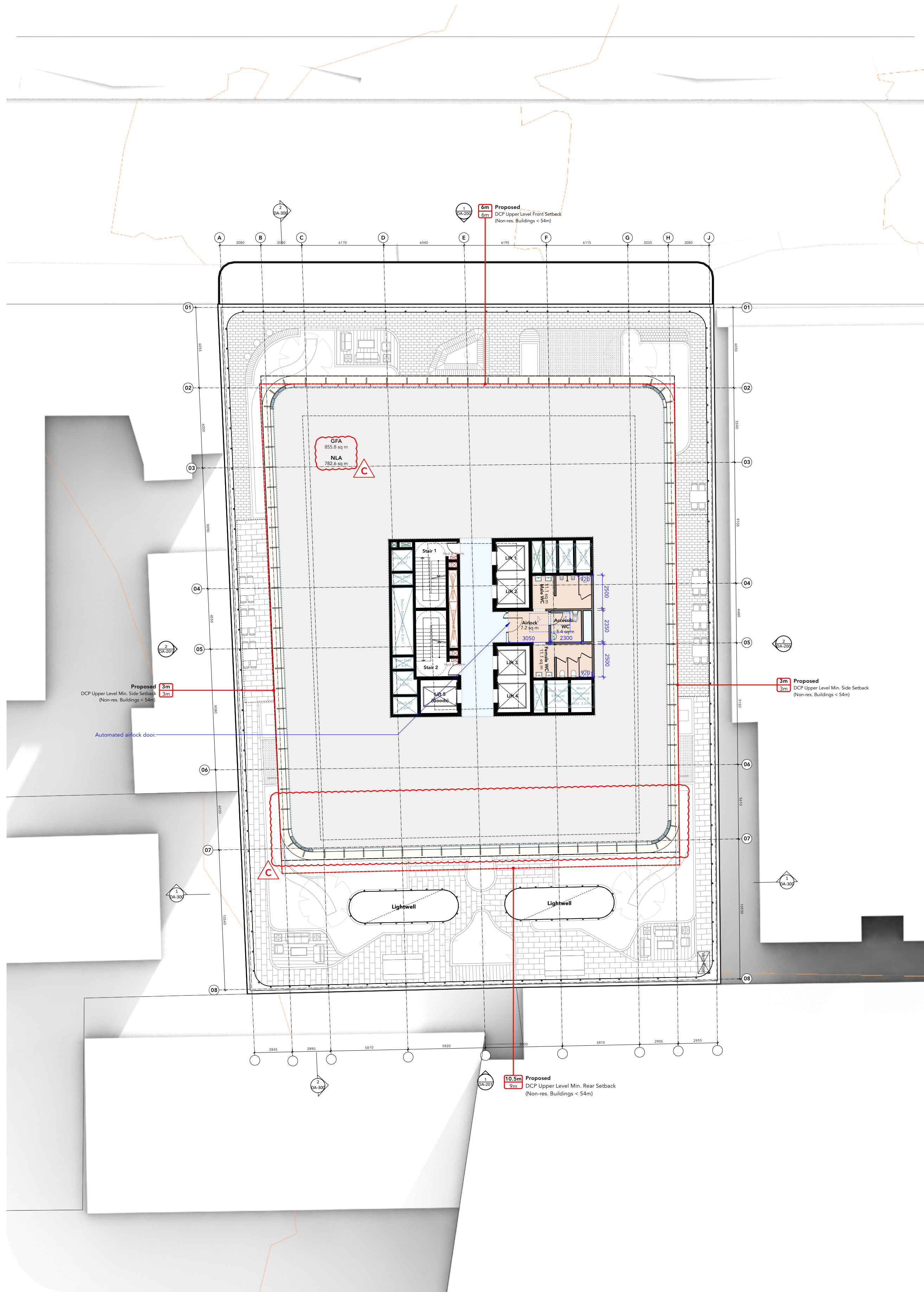
1 Plan-Tower-Levels 11-12 Scale: 1:200
