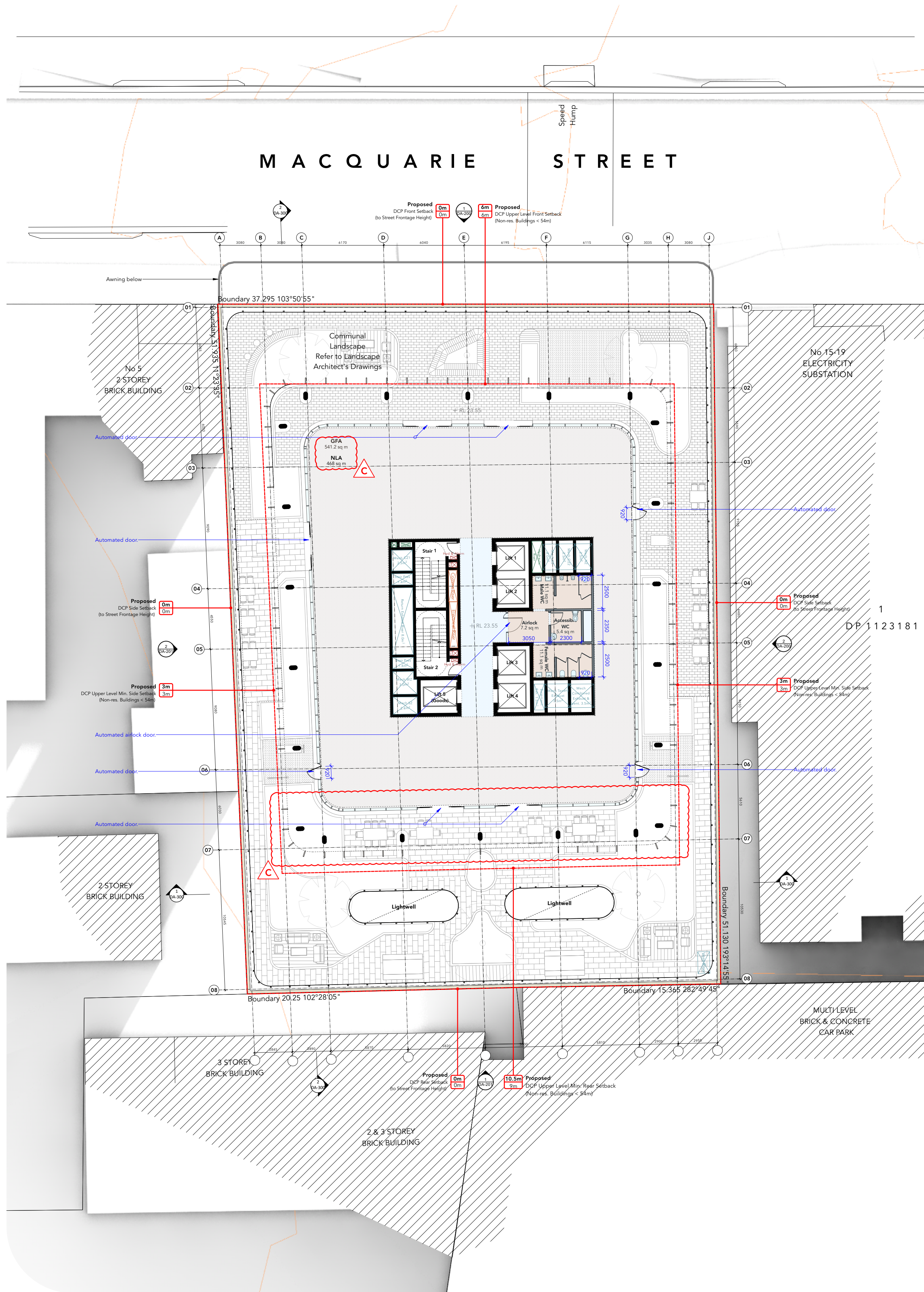
1 Plan-Tower-Level 4 Scale: 1:200
